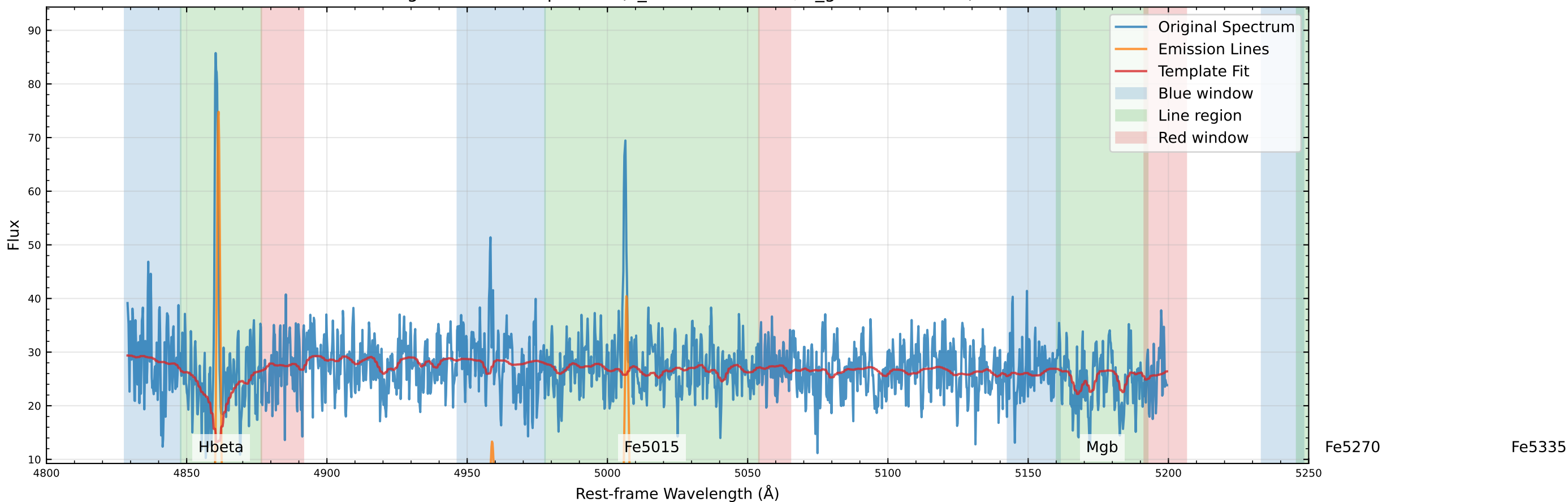
Original Data Comparison (v_star=-39.4 km/s, v_gas=-43.7 km/s)
