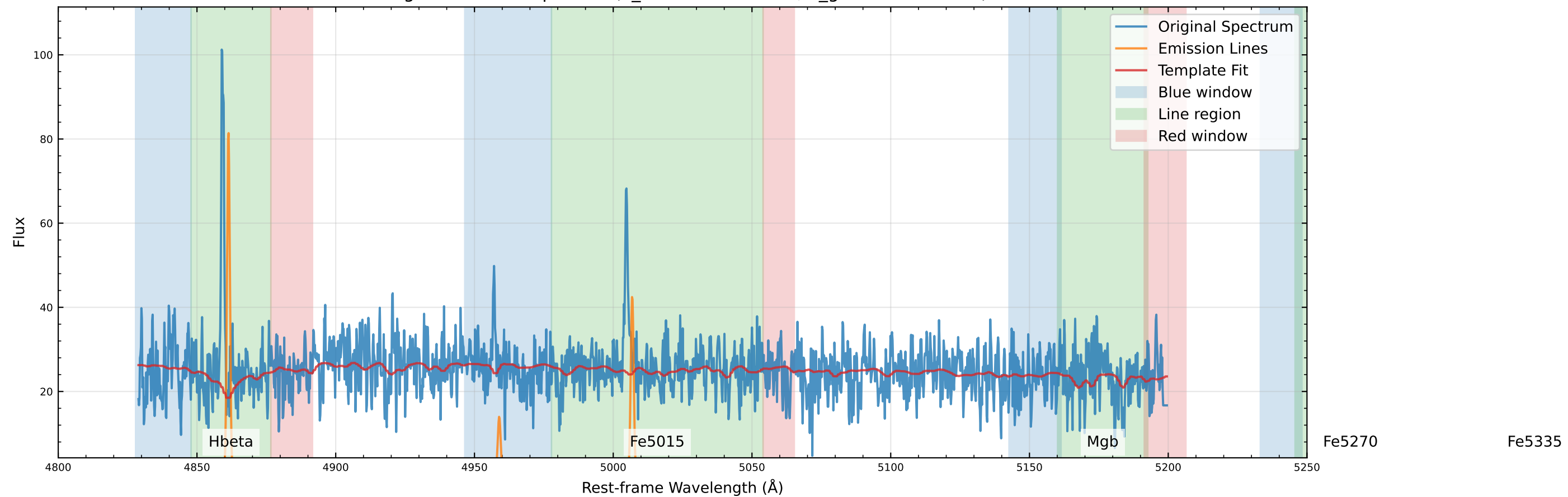
Original Data Comparison (v_star=-163.3 km/s, v_gas=-128.8 km/s)
