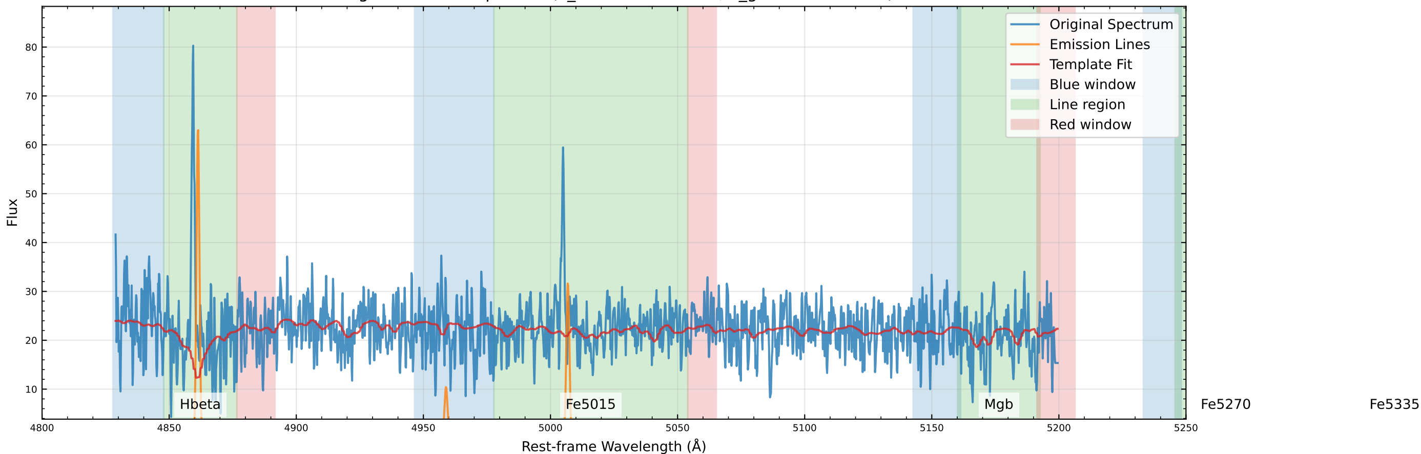
Original Data Comparison (v_star=-114.4 km/s, v_gas=-120.7 km/s)
