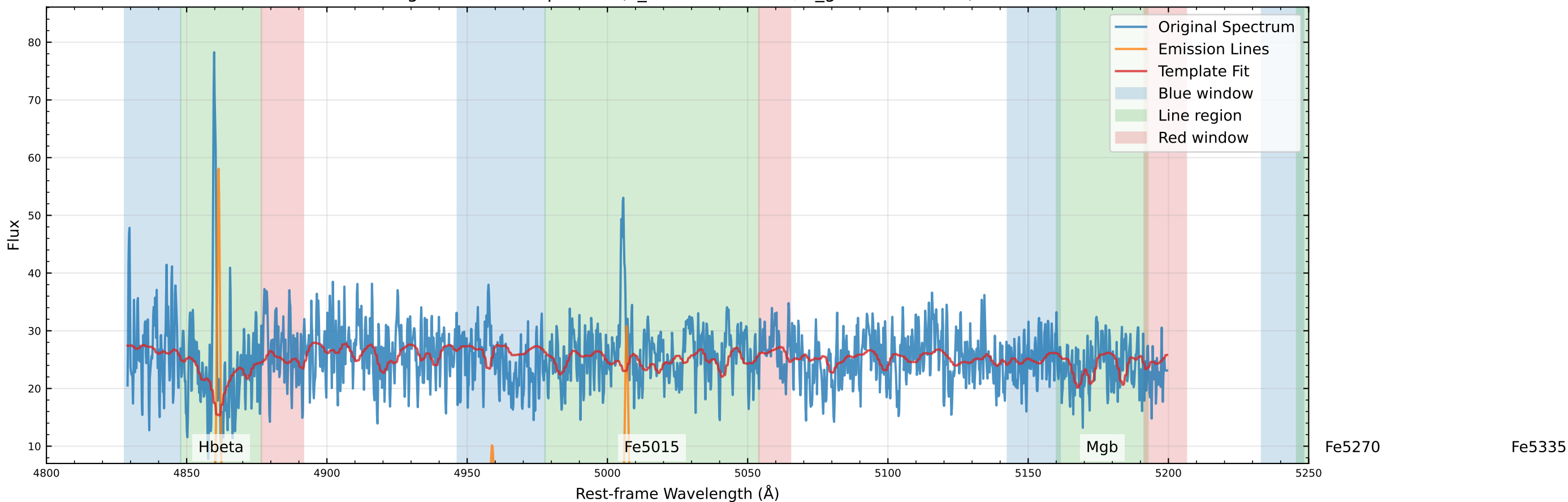
Original Data Comparison (v_star=-85.9 km/s, v_gas=-85.9 km/s)
