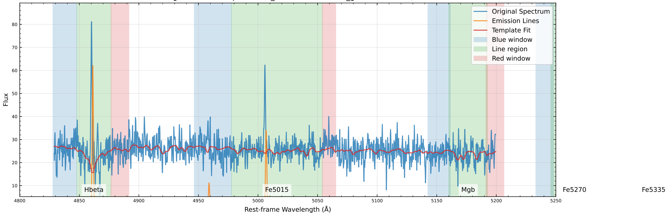
Original Data Comparison (v_star=-74.7 km/s, v_gas=-66.9 km/s)
