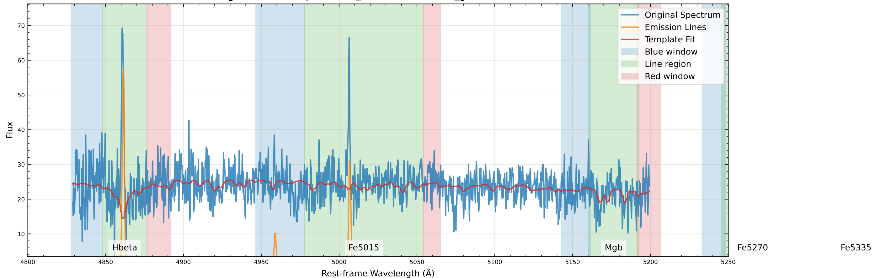
Original Data Comparison (v_star=-38.1 km/s, v_gas=-29.9 km/s)
