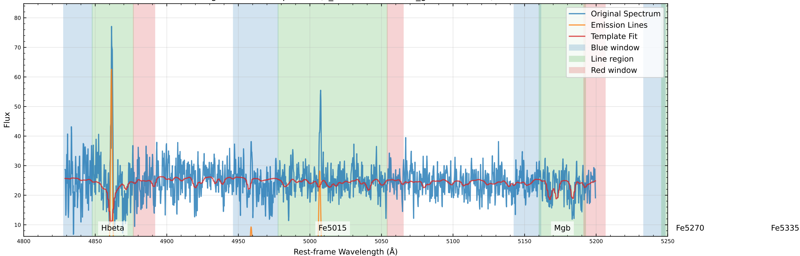
Original Data Comparison (v_star=26.7 km/s, v_gas=17.3 km/s)
