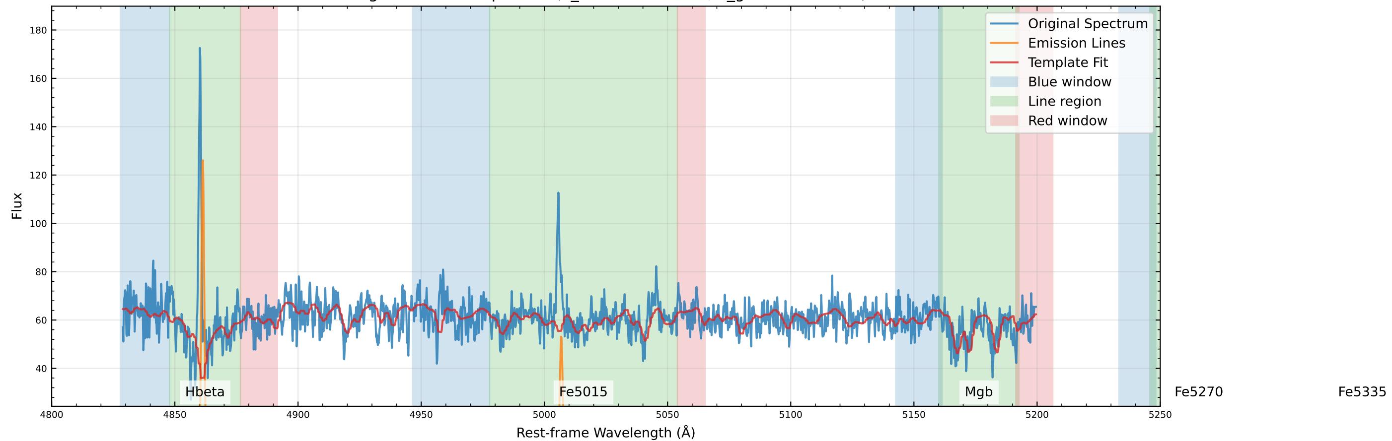
Original Data Comparison (v_star=-60.1 km/s, v_gas=-71.5 km/s)
