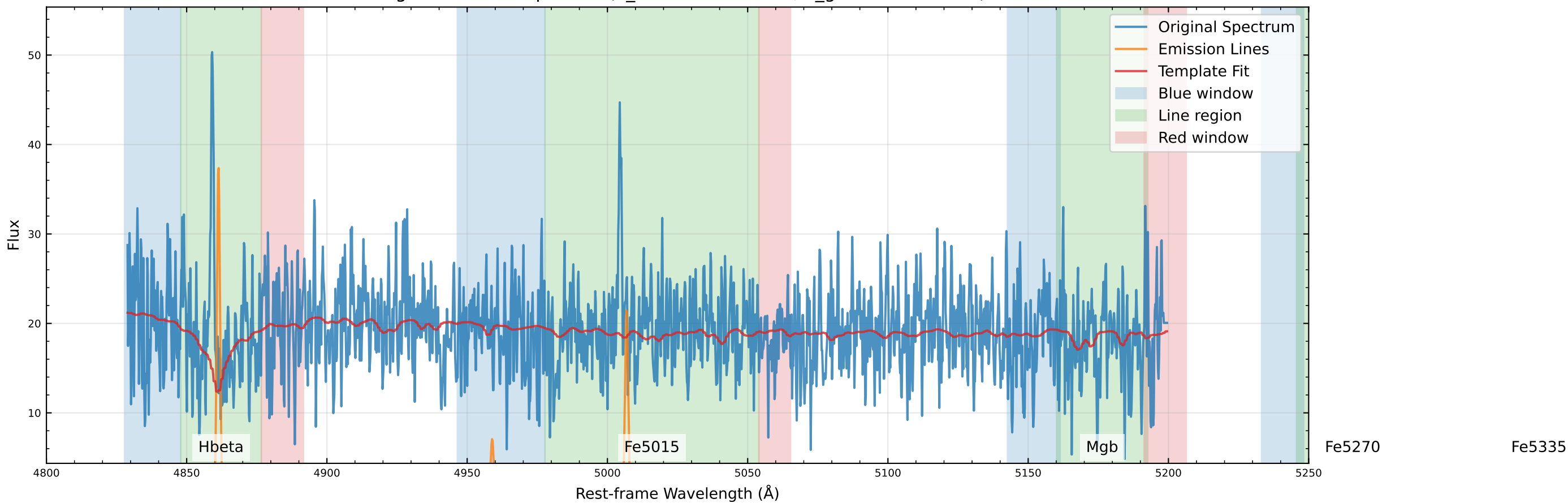
Original Data Comparison (v_star=-148.2 km/s, v_gas=-139.2 km/s)
