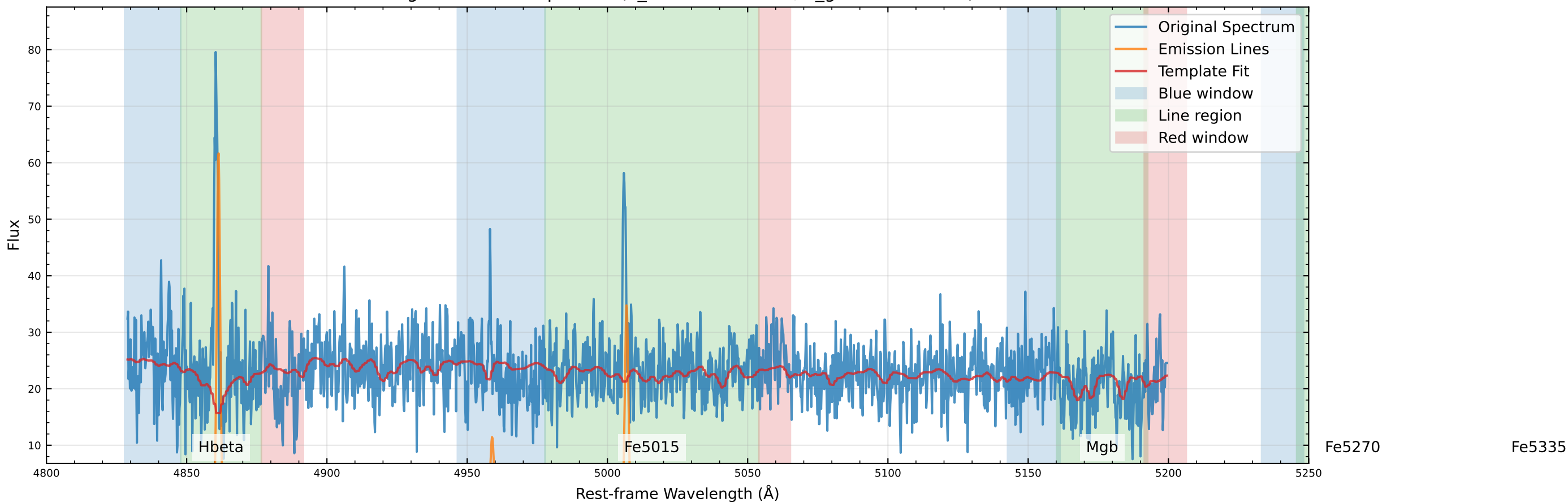
Original Data Comparison (v_star=-64.4 km/s, v_gas=-54.5 km/s)
