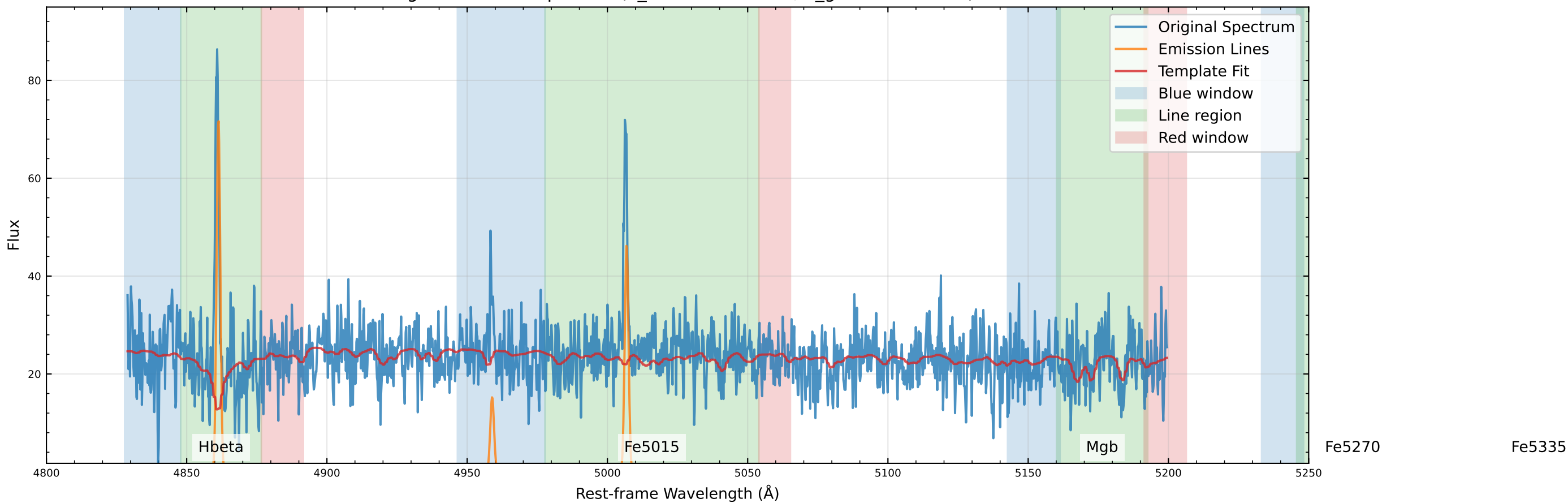
Original Data Comparison (v_star=-15.8 km/s, v_gas=-29.2 km/s)
