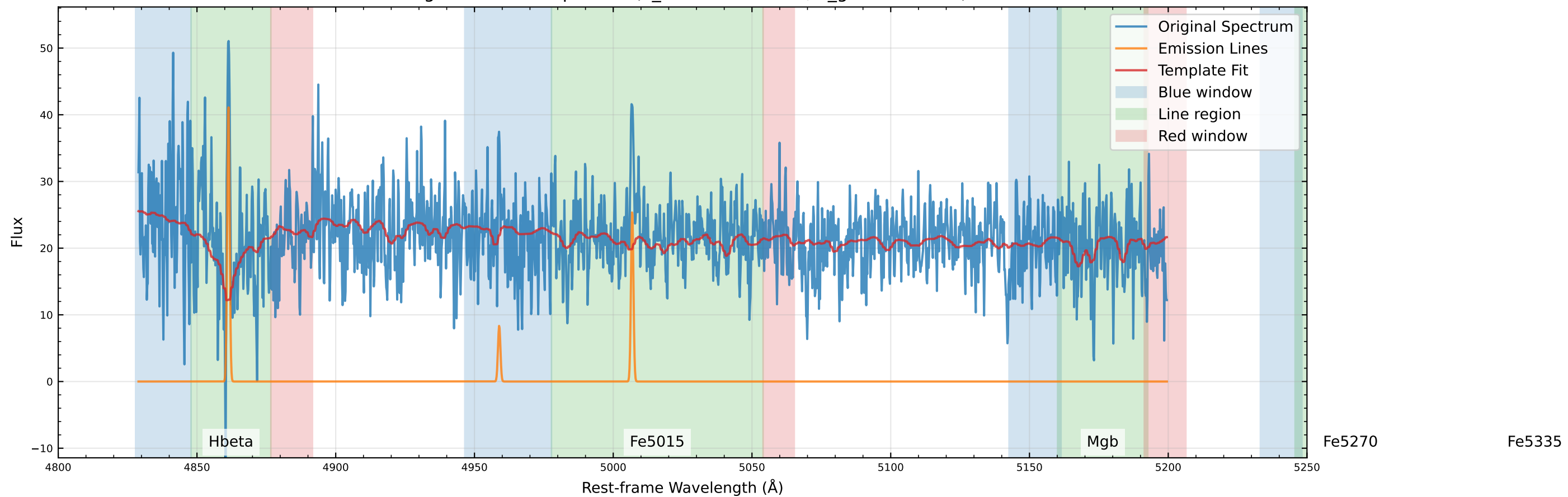
Original Data Comparison (v_star=-24.4 km/s, v_gas=1.3 km/s)
