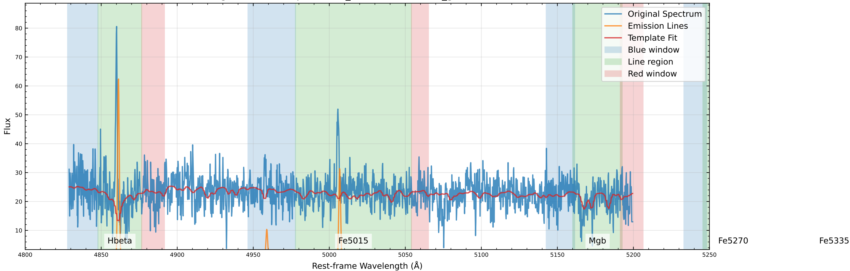
Original Data Comparison (v_star=-55.8 km/s, v_gas=-78.8 km/s)
