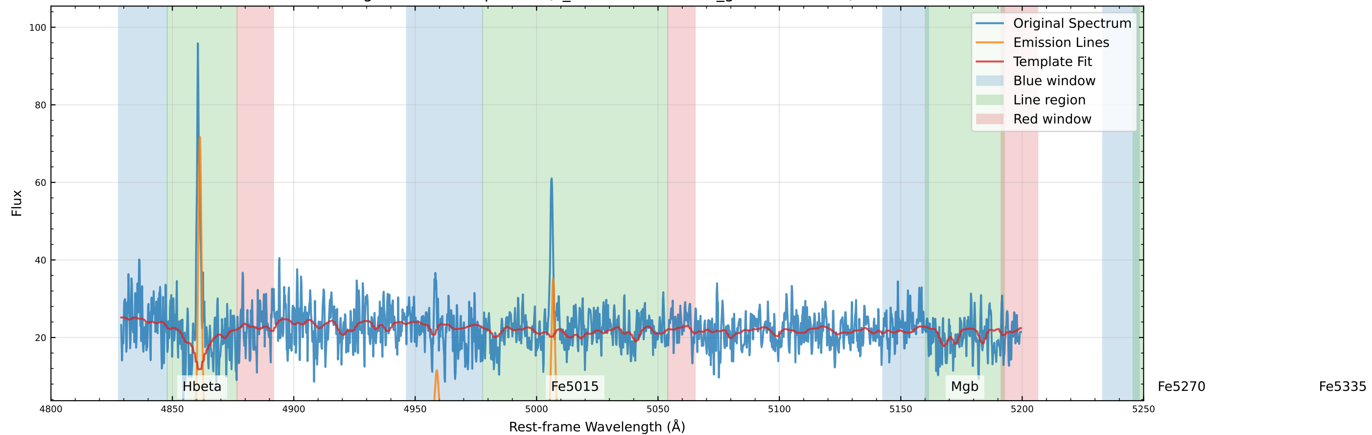
Original Data Comparison (v_star=-60.7 km/s, v_gas=-40.1 km/s)
