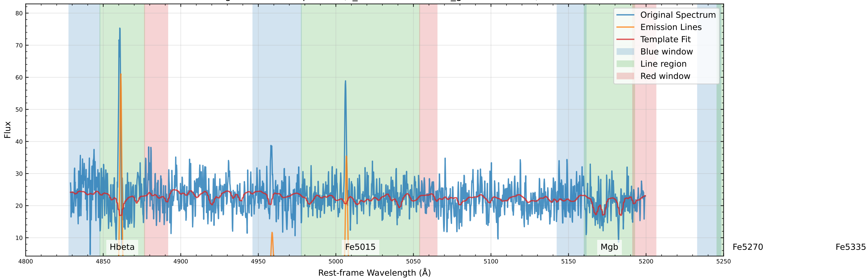
Original Data Comparison (v_star=-37.0 km/s, v_gas=-44.7 km/s)
