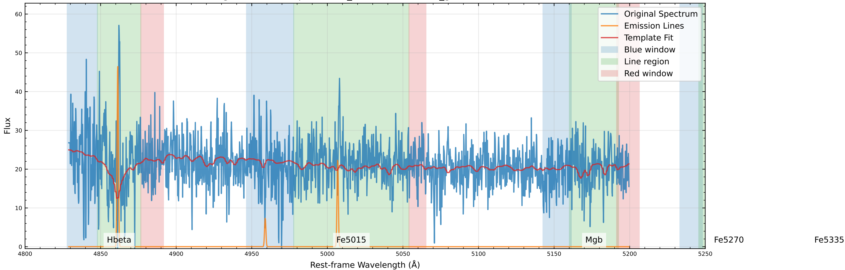
Original Data Comparison (v_star=63.6 km/s, v_gas=58.9 km/s)
