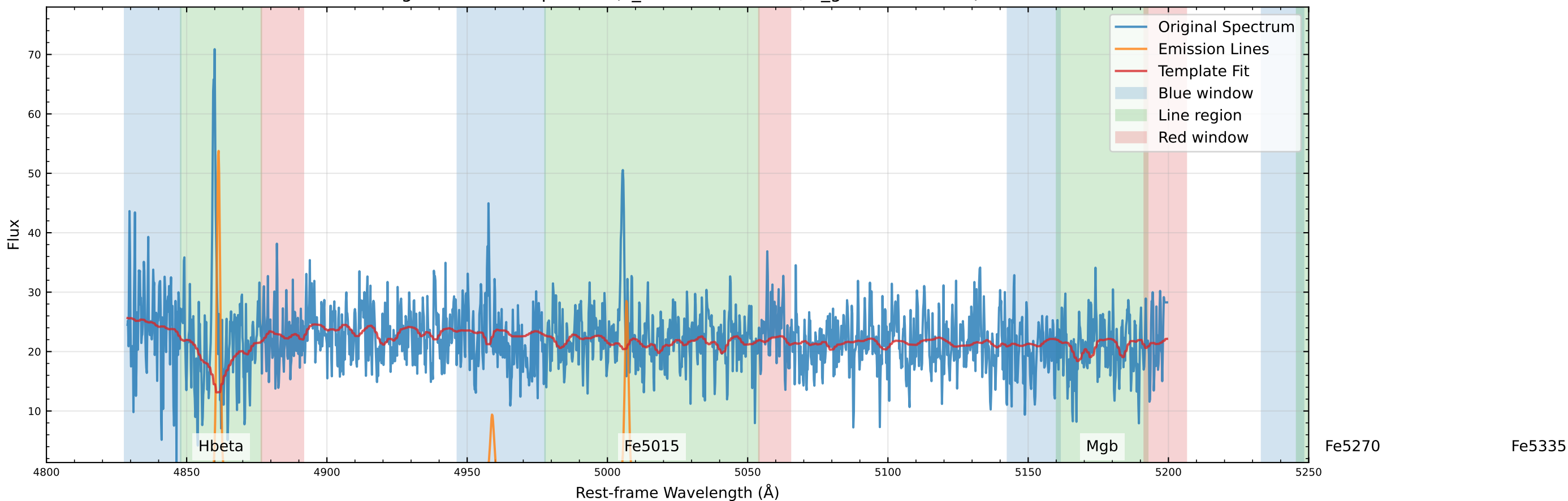
Original Data Comparison (v_star=-113.7 km/s, v_gas=-94.8 km/s)
