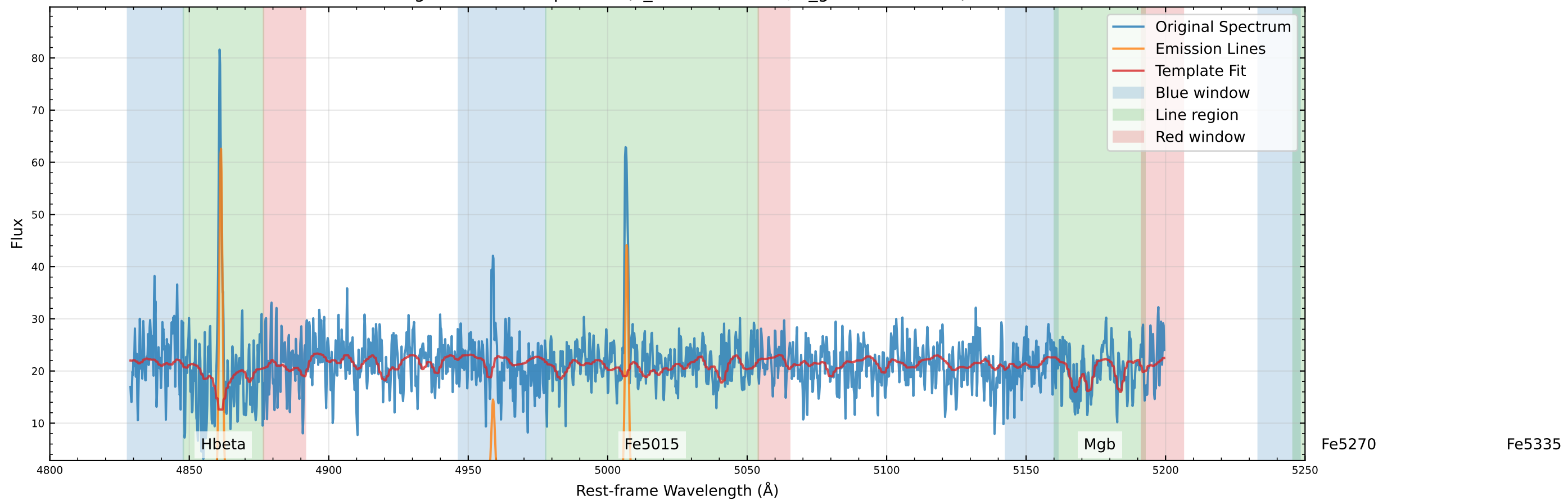
Original Data Comparison (v_star=-6.9 km/s, v_gas=-16.8 km/s)
