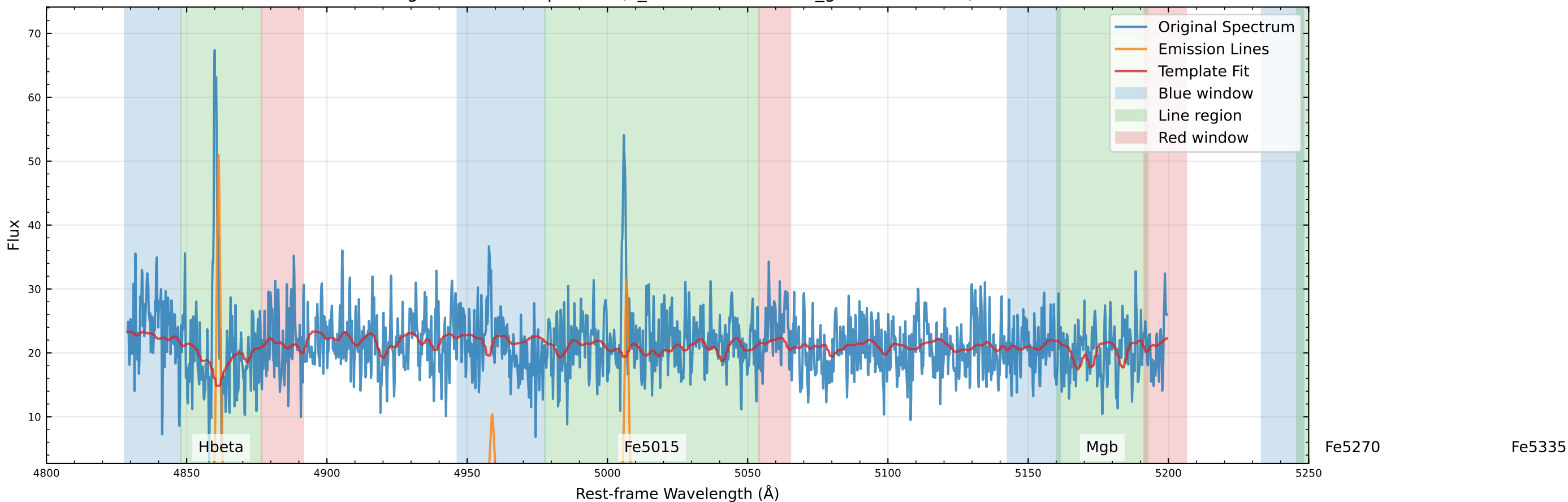
Original Data Comparison (v_star=-57.2 km/s, v_gas=-63.5 km/s)
