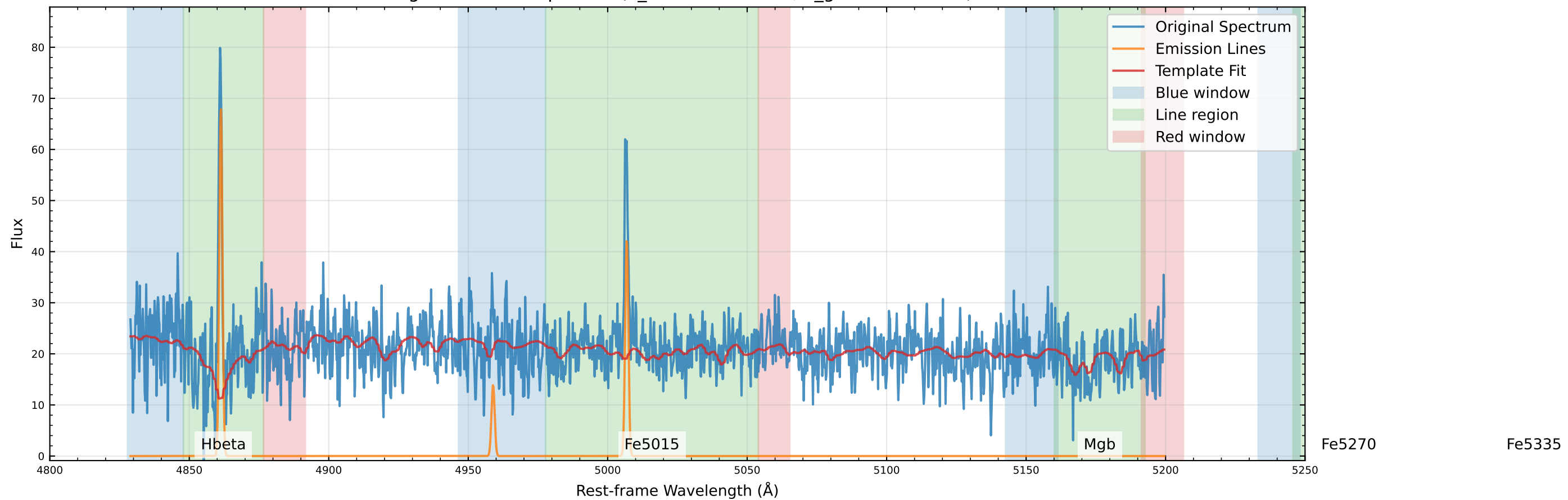
Original Data Comparison (v_star=-11.0 km/s, v_gas=-14.8 km/s)
