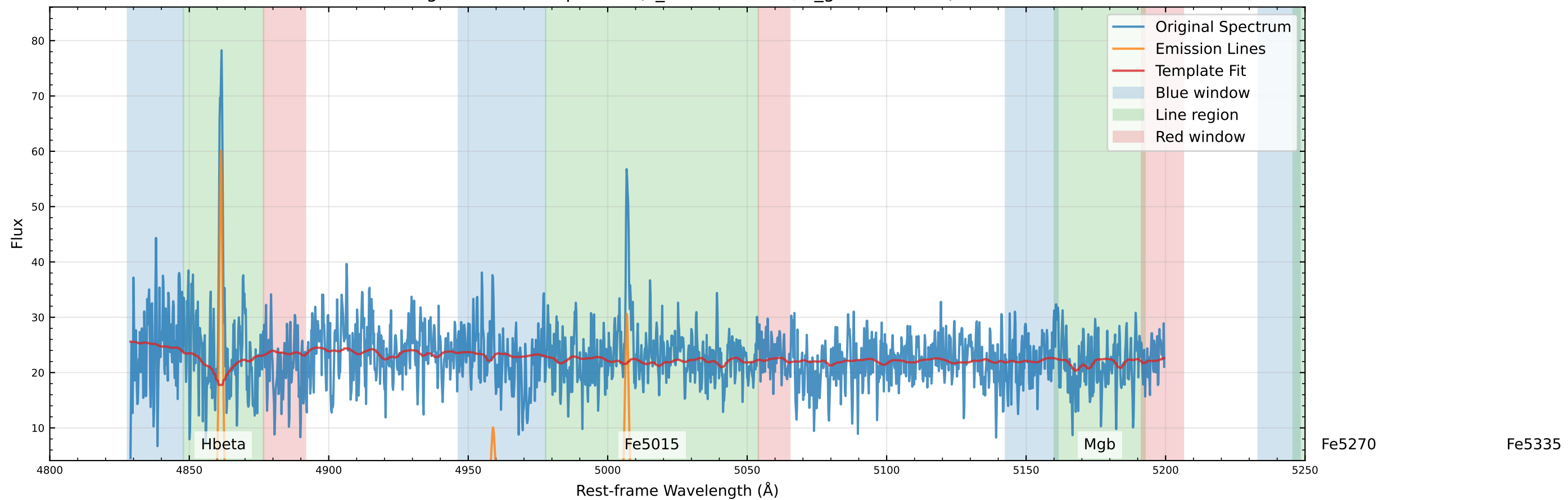
Original Data Comparison (v_star=8.5 km/s, v_gas=5.1 km/s)
