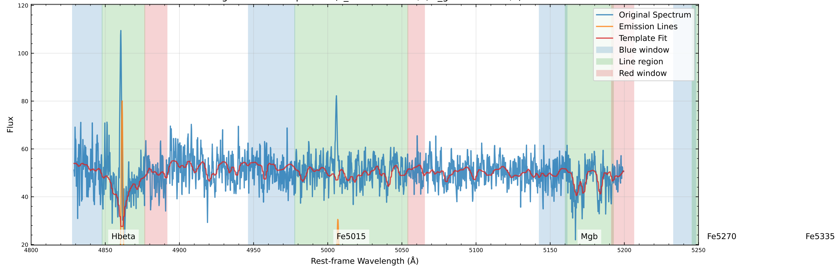
Original Data Comparison (v_star=-64.3 km/s, v_gas=-60.5 km/s)
