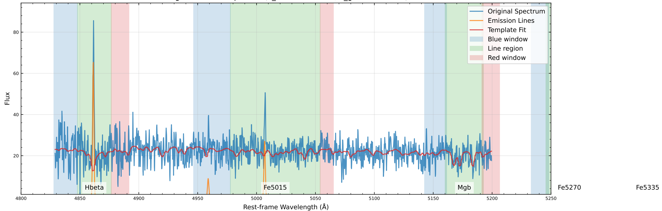
Original Data Comparison (v_star=14.6 km/s, v_gas=13.8 km/s)
