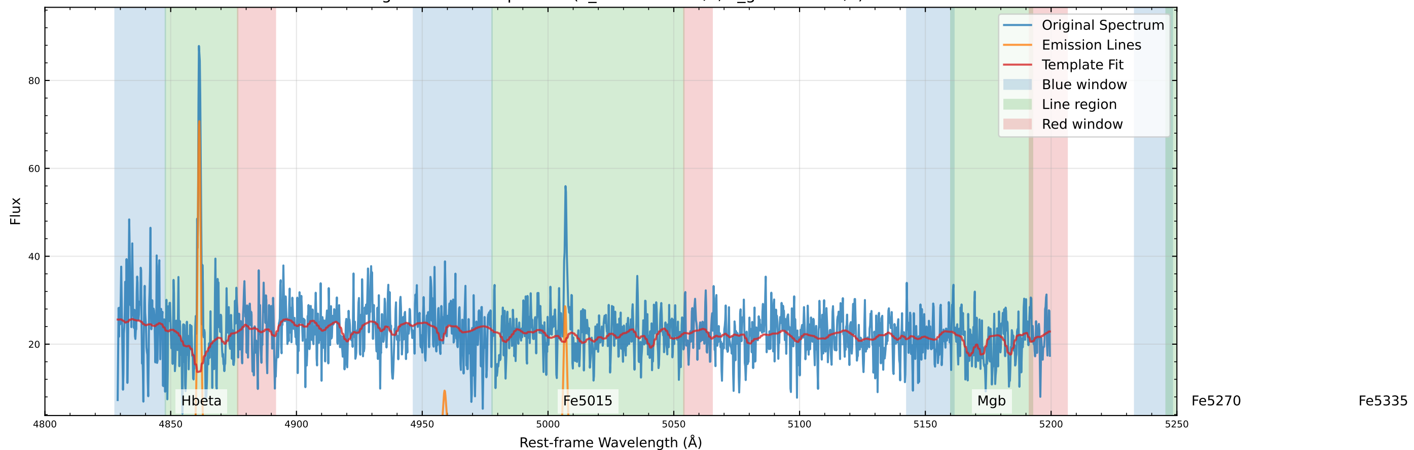
Original Data Comparison (v_star=-1.4 km/s, v_gas=5.5 km/s)
