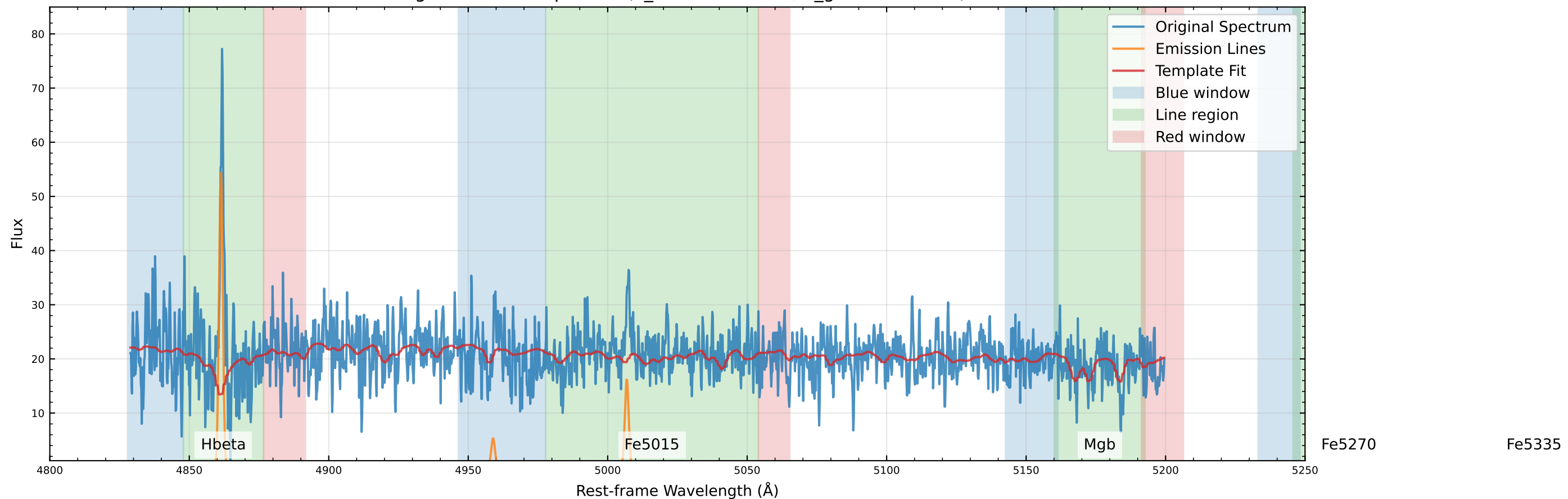
Original Data Comparison (v_star=47.5 km/s, v_gas=26.4 km/s)
