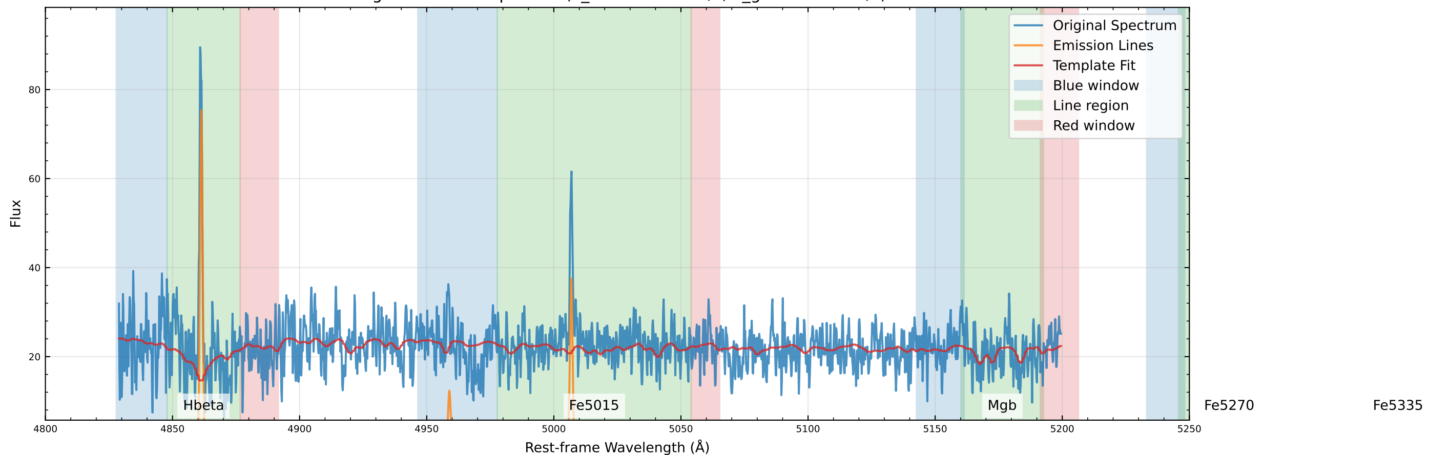
Original Data Comparison (v_star=-27.6 km/s, v_gas=-11.6 km/s)
