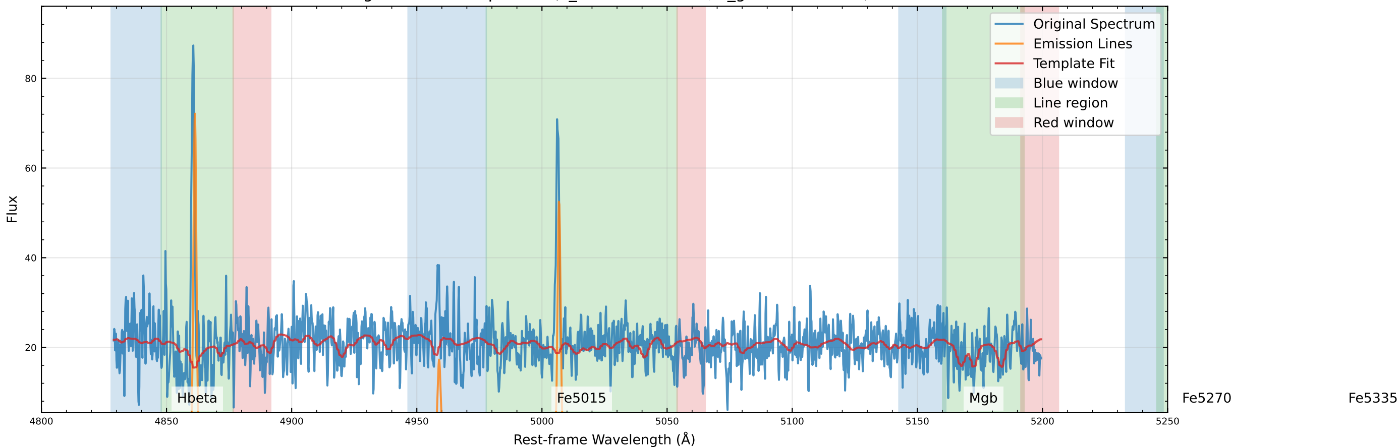
Original Data Comparison (v_star=-37.1 km/s, v_gas=-43.1 km/s)
