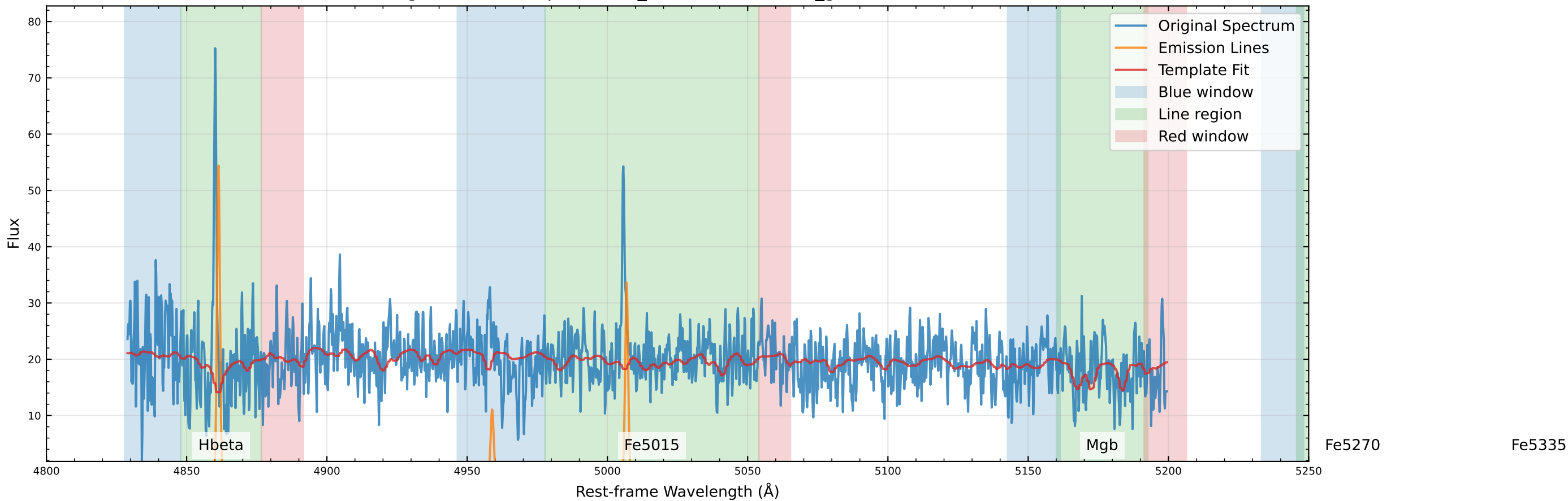
Original Data Comparison (v_star=-81.1 km/s, v_gas=-72.0 km/s)
