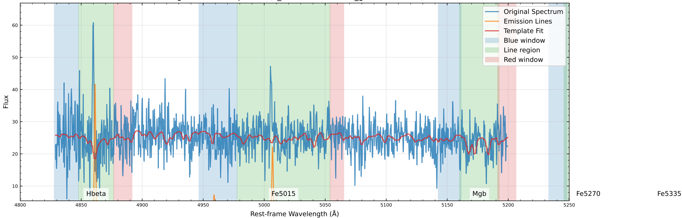
Original Data Comparison (v_star=-86.9 km/s, v_gas=-91.3 km/s)
