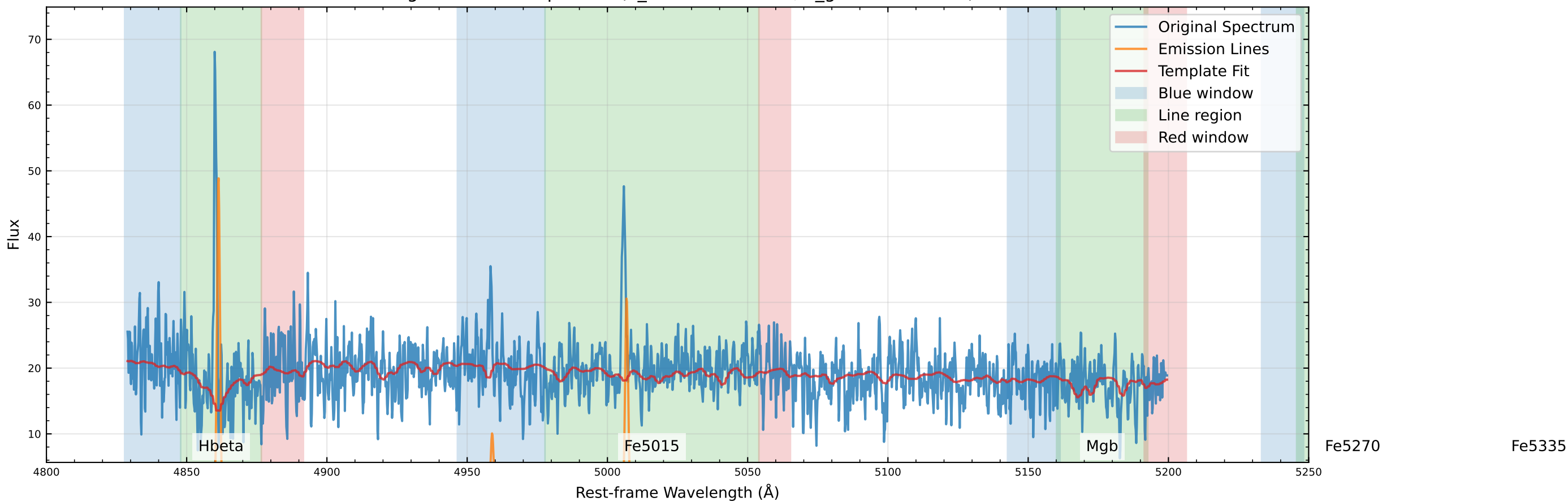
Original Data Comparison (v_star=-91.0 km/s, v_gas=-67.4 km/s)
