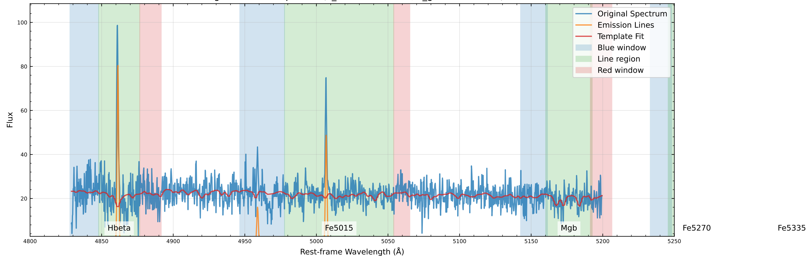
Original Data Comparison (v_star=-36.6 km/s, v_gas=-16.6 km/s)
