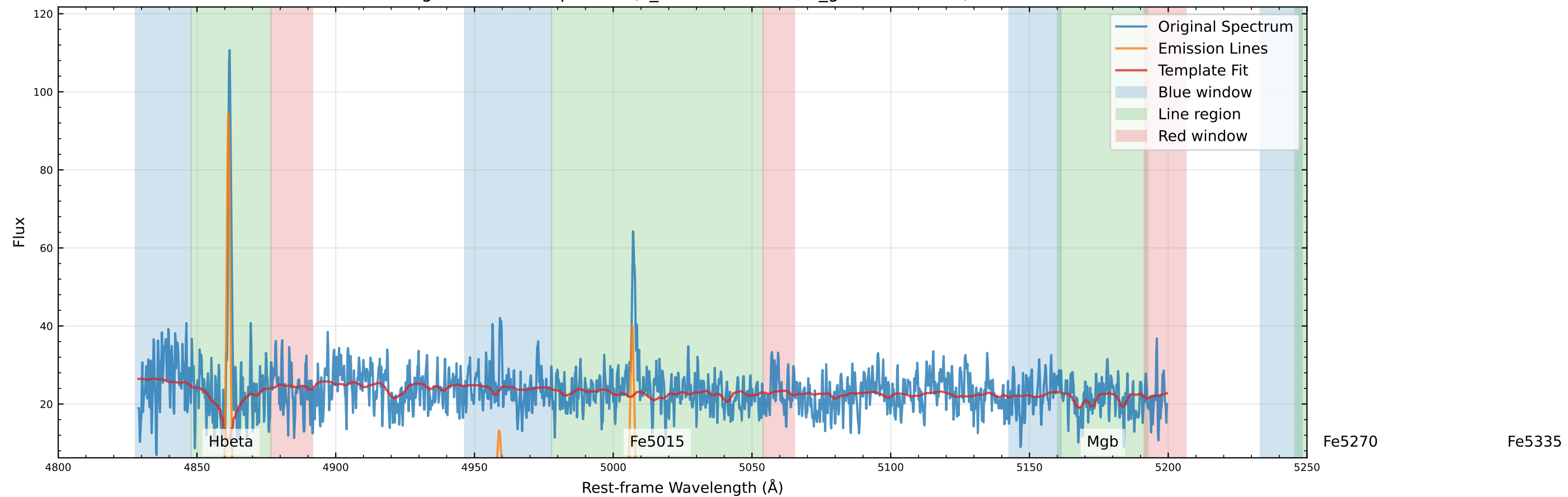
Original Data Comparison (v_star=34.5 km/s, v_gas=28.4 km/s)
