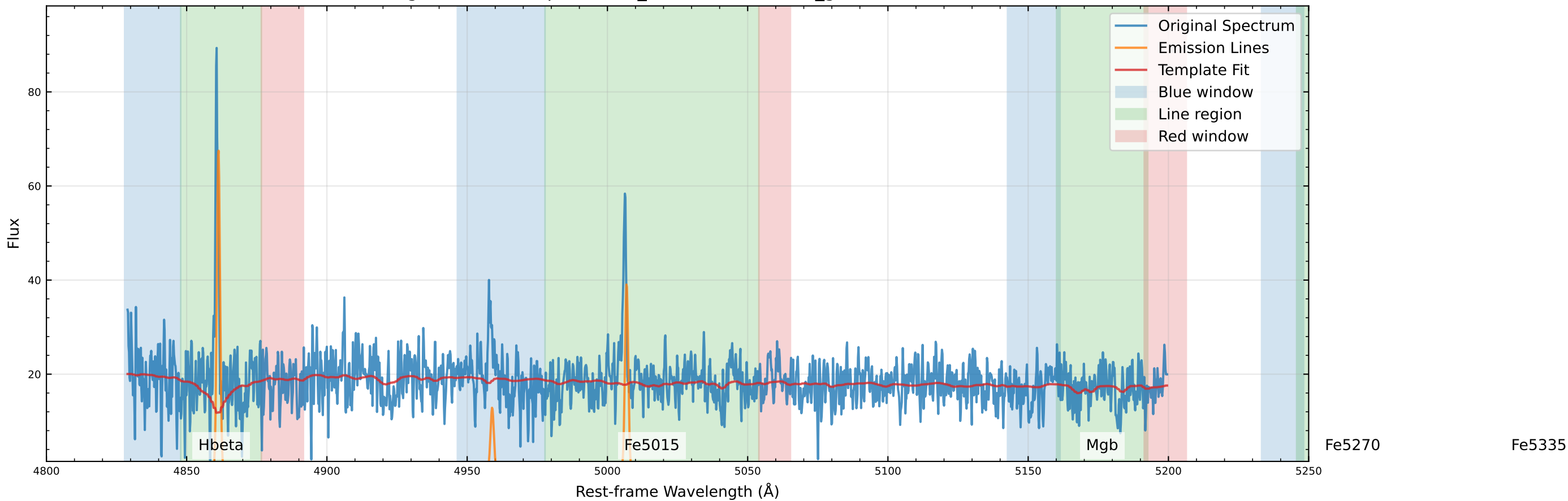
Original Data Comparison (v_star=-48.1 km/s, v_gas=-39.4 km/s)
