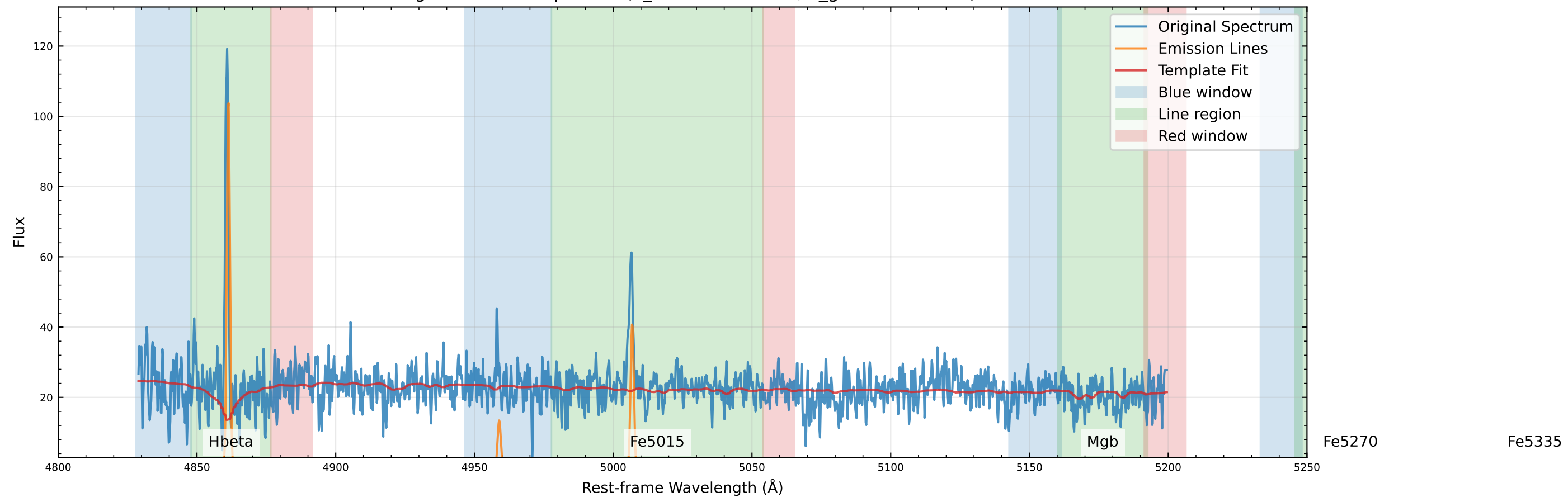
Original Data Comparison (v_star=-80.6 km/s, v_gas=-36.5 km/s)
