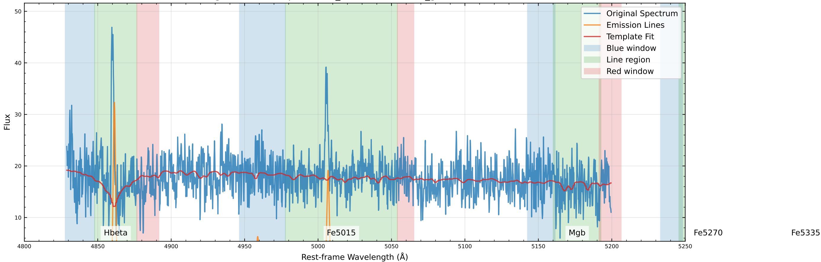
Original Data Comparison (v_star=40.6 km/s, v_gas=-73.5 km/s)
