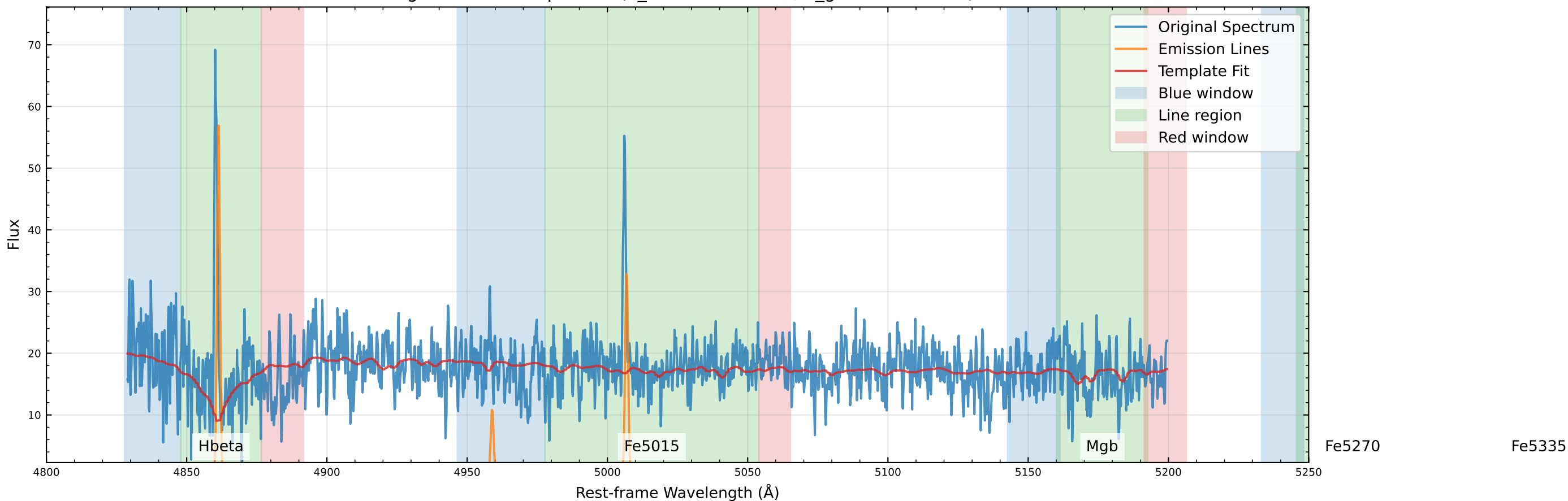
Original Data Comparison (v_star=-48.9 km/s, v_gas=-53.8 km/s)
