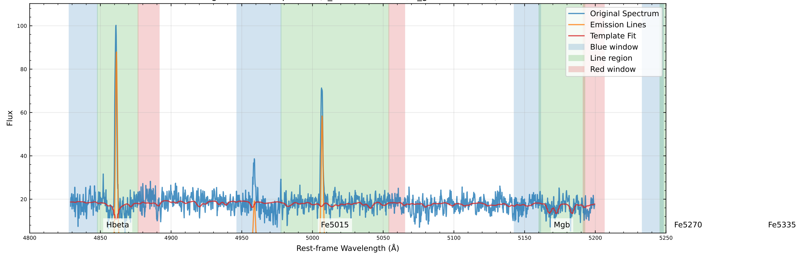
Original Data Comparison (v_star=-12.4 km/s, v_gas=-22.9 km/s)
