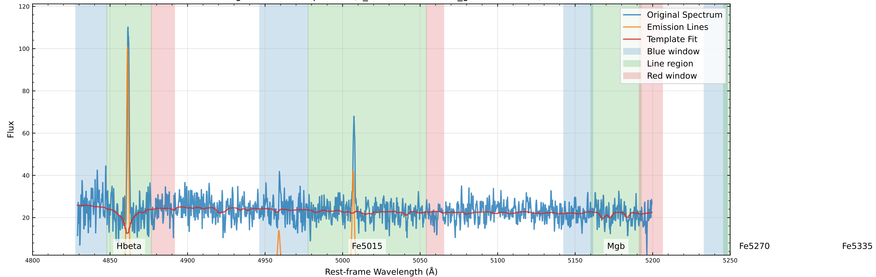
Original Data Comparison (v_star=31.0 km/s, v_gas=25.8 km/s)
