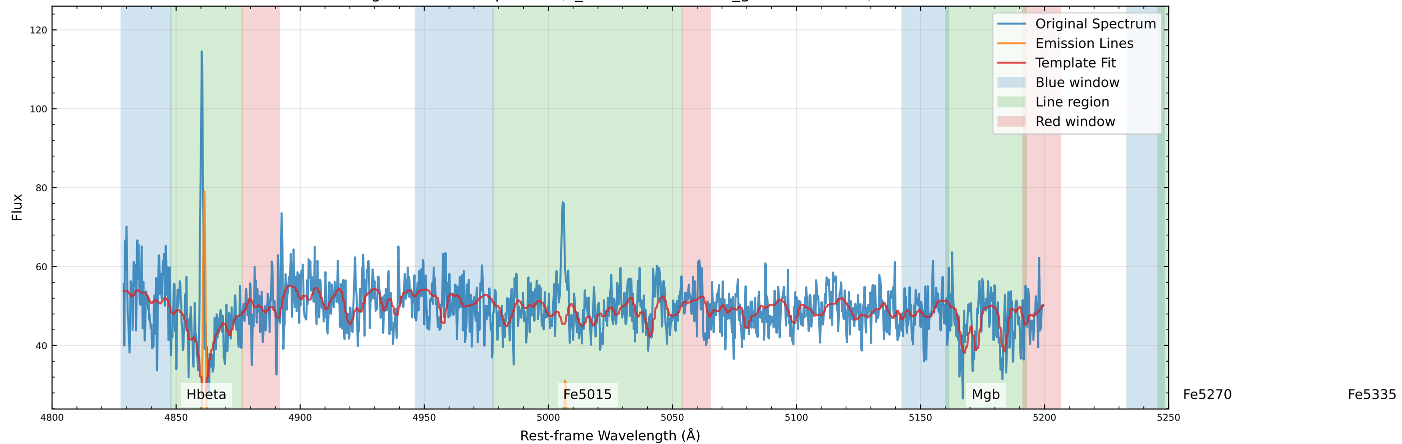
Original Data Comparison (v_star=-71.2 km/s, v_gas=-60.9 km/s)
