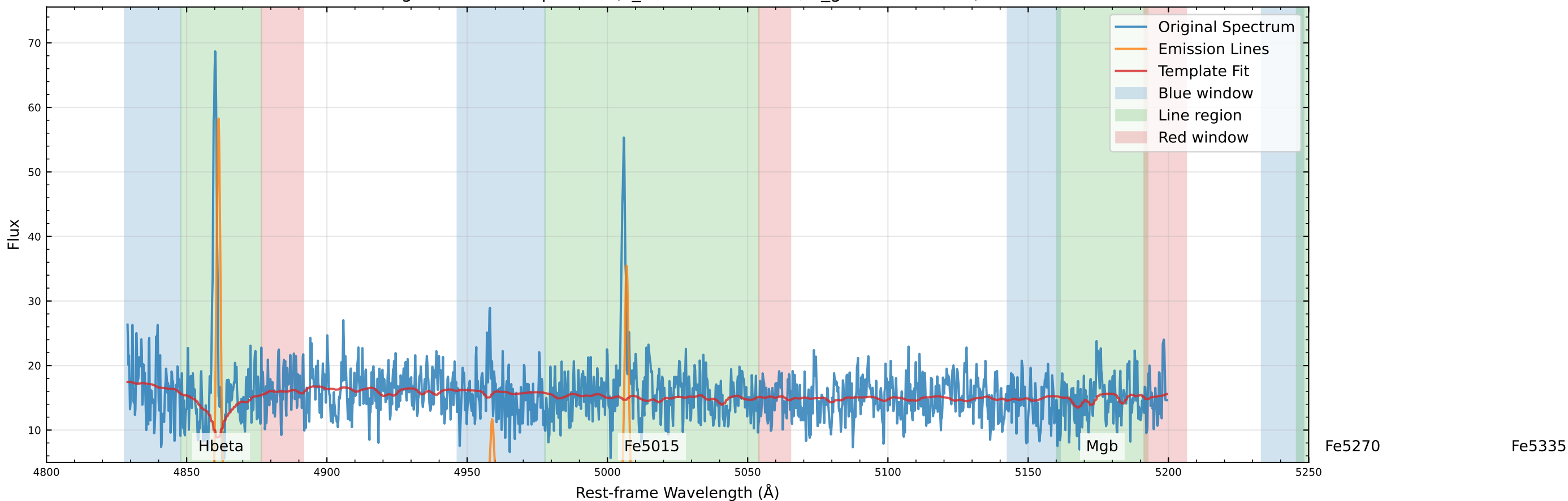
Original Data Comparison (v_star=-100.2 km/s, v_gas=-73.1 km/s)
