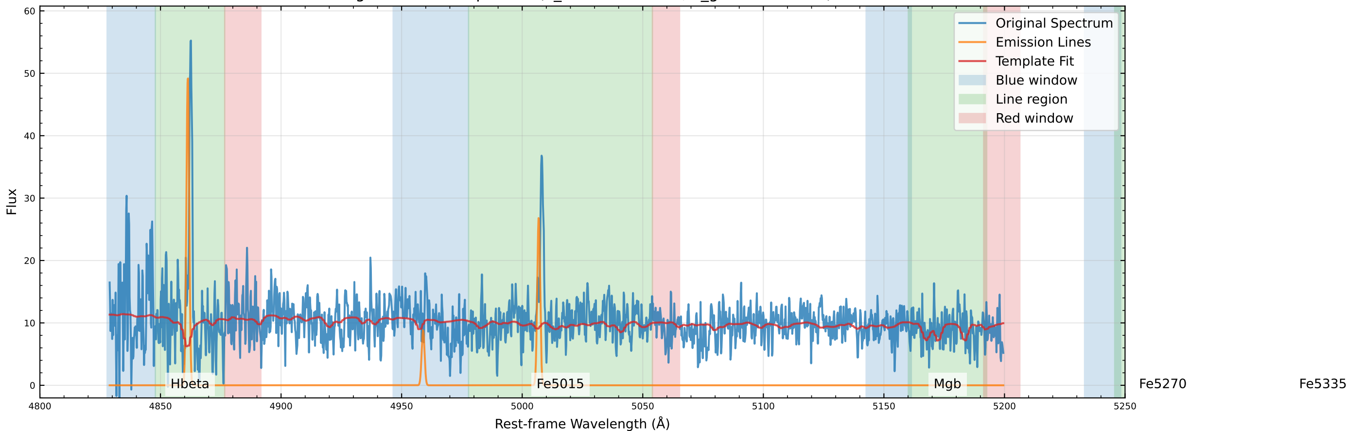
Original Data Comparison (v_star=80.4 km/s, v_gas=74.6 km/s)
