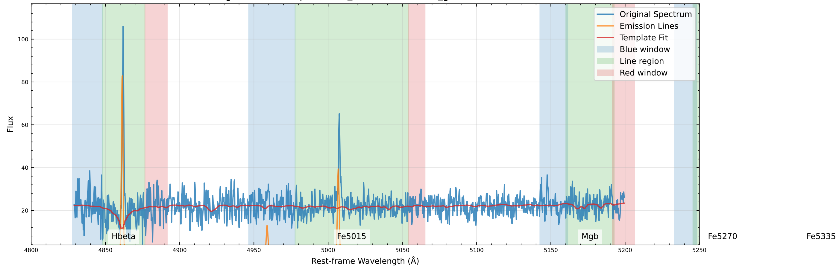
Original Data Comparison (v_star=66.1 km/s, v_gas=36.3 km/s)
