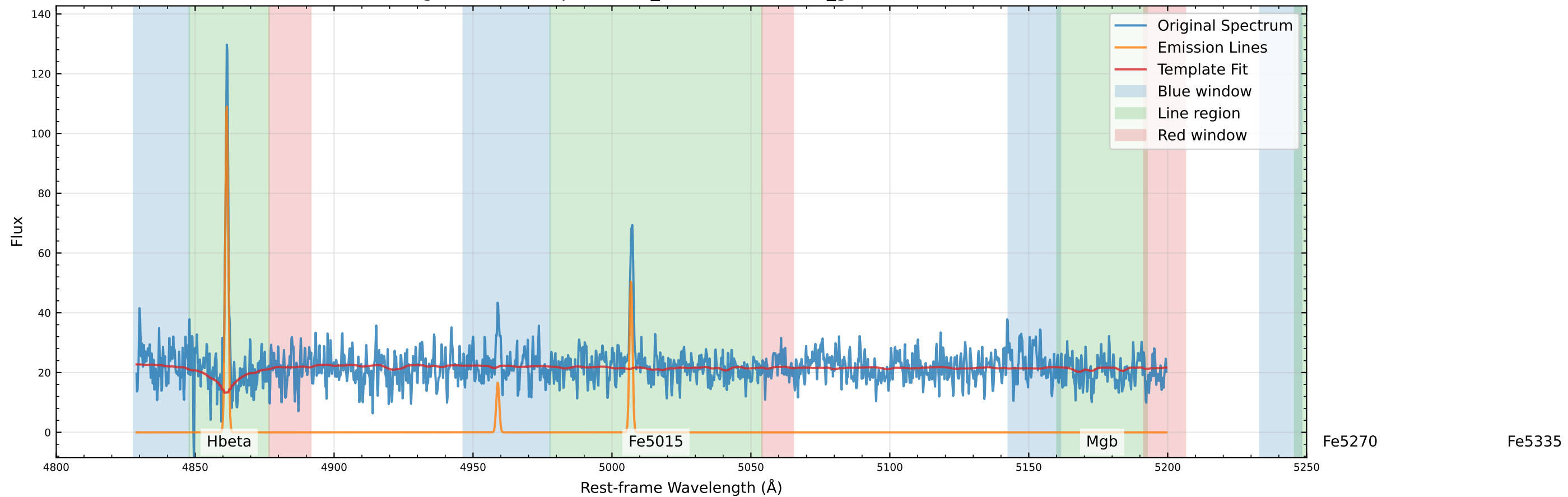
Original Data Comparison (v_star=-12.8 km/s, v_gas=7.9 km/s)
