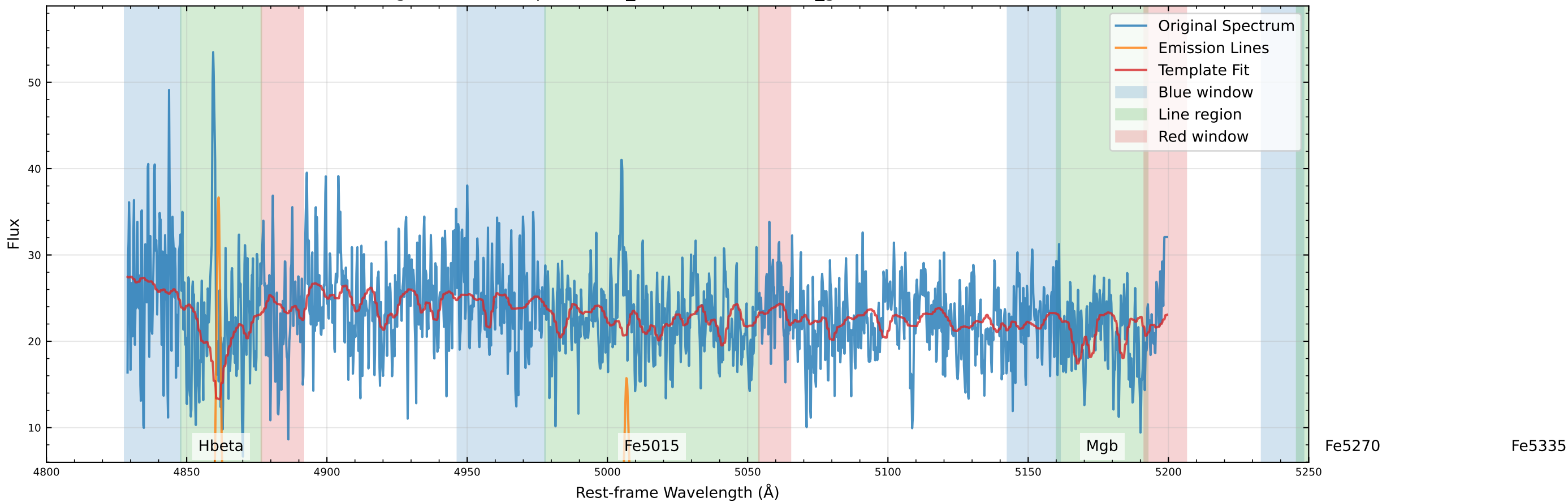
Original Data Comparison (v_star=-112.4 km/s, v_gas=-113.4 km/s)
