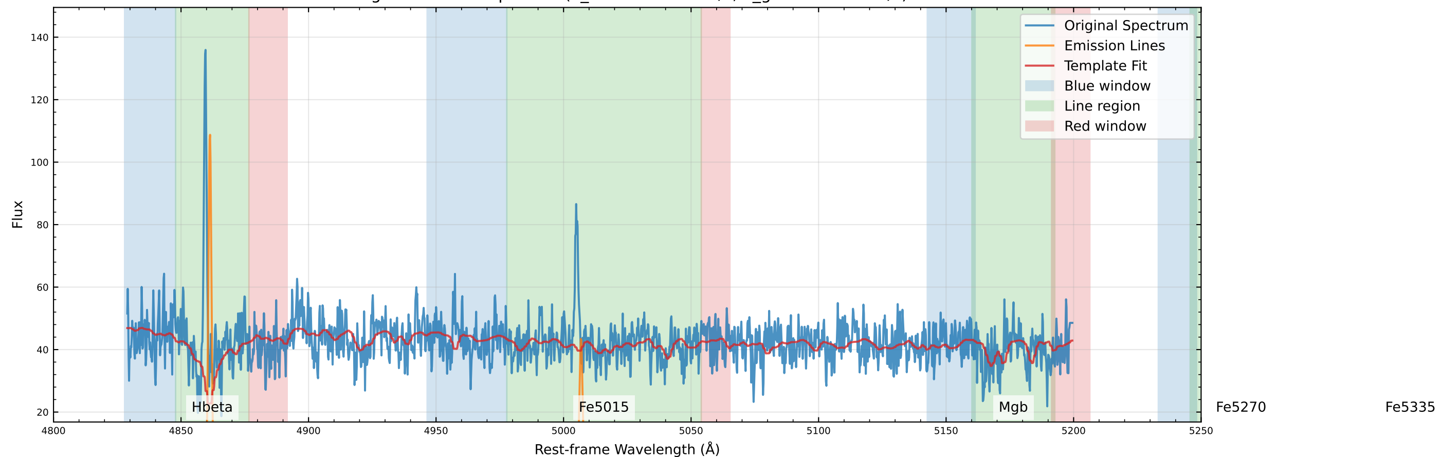
Original Data Comparison (v_star=-110.8 km/s, v_gas=-112.4 km/s)
