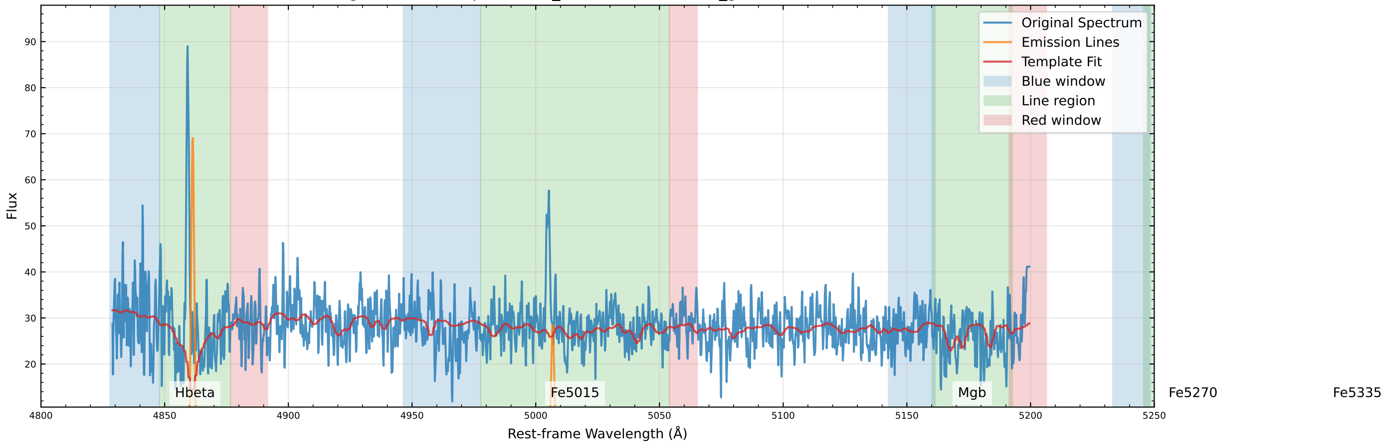
Original Data Comparison (v_star=-119.7 km/s, v_gas=-123.4 km/s)
