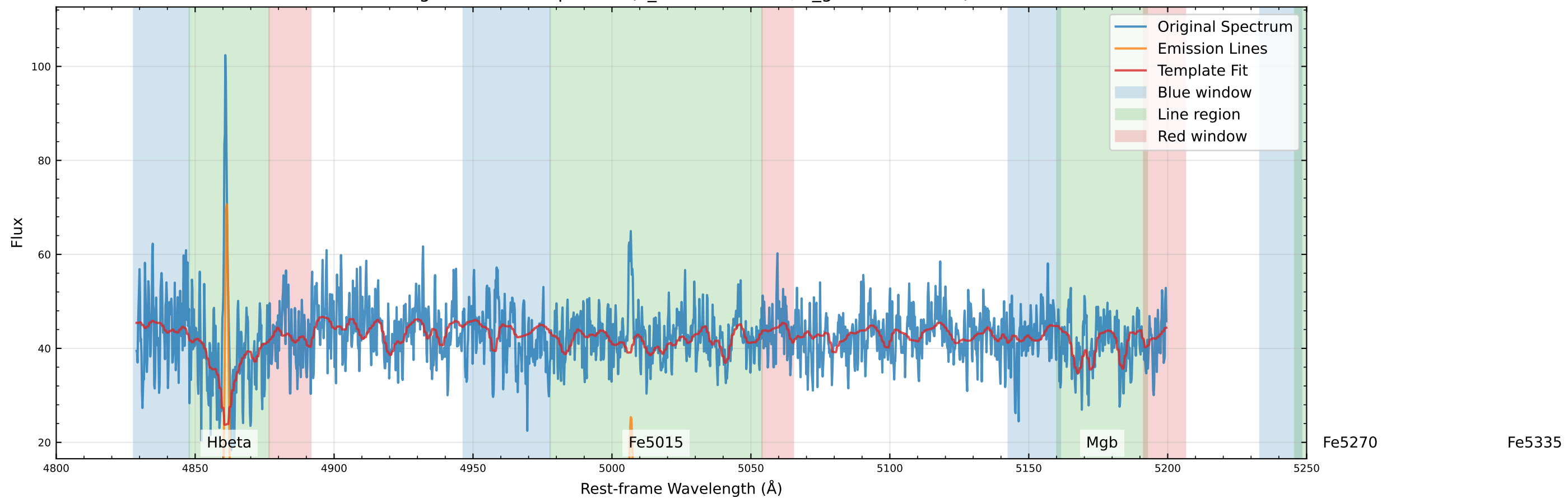
Original Data Comparison ( v_{\text{star}}=-7.5 km/s, v_{\text{gas}}=-22.3 km/s)
