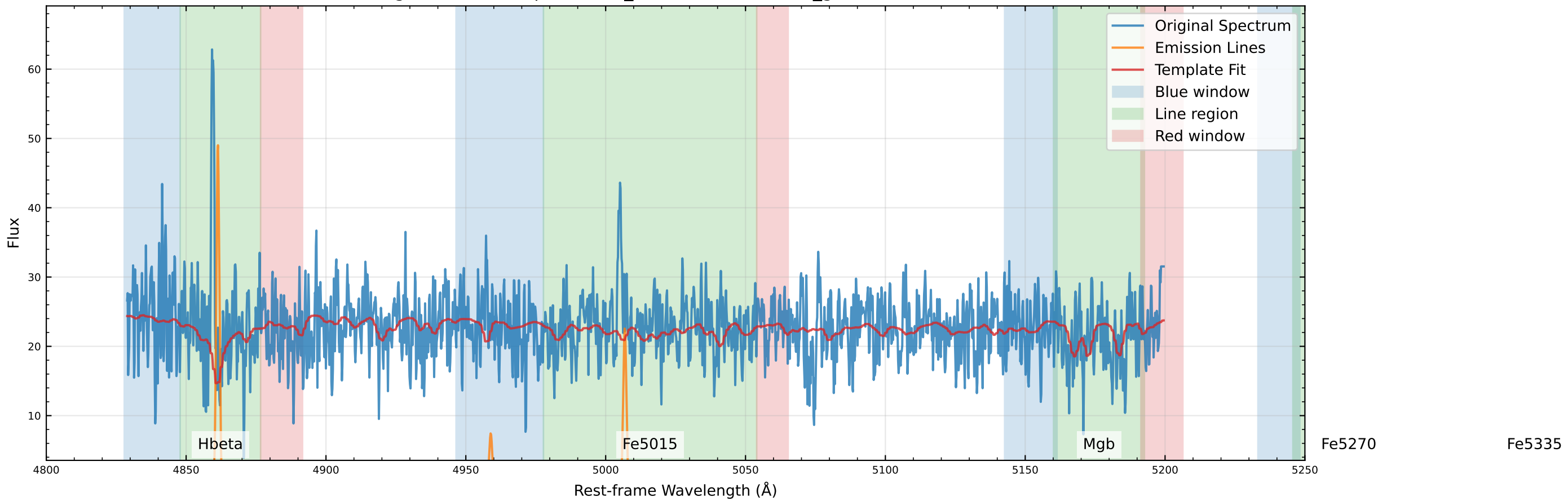
Original Data Comparison (v_star=-104.8 km/s, v_gas=-112.5 km/s)
