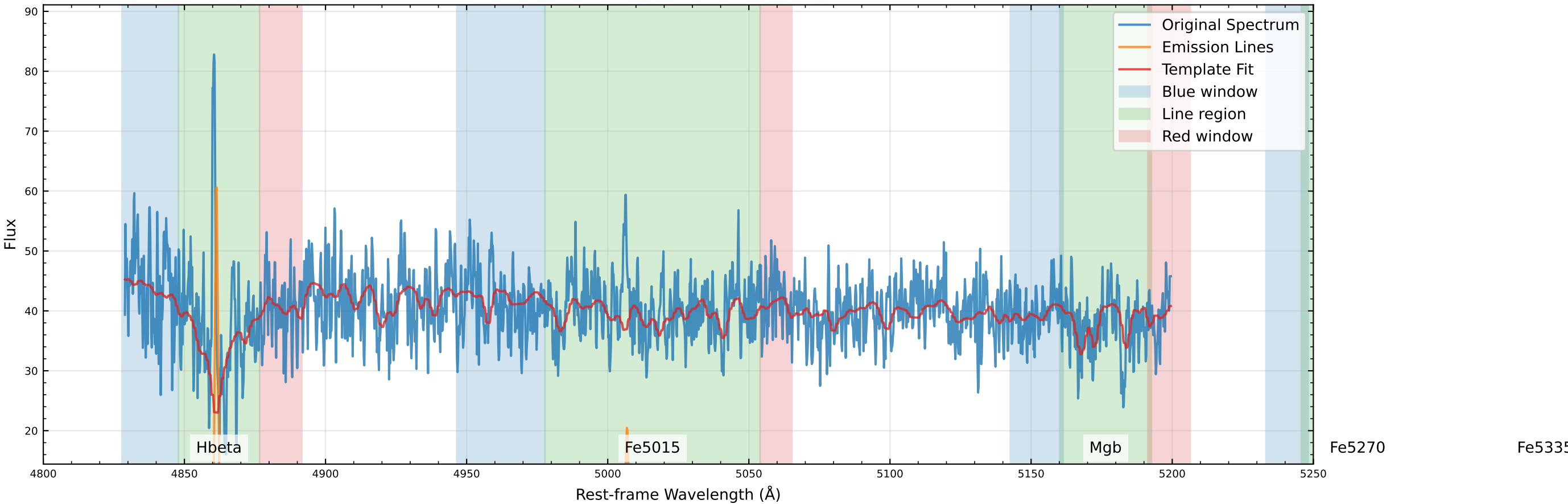
Original Data Comparison (v_star=-49.8 km/s, v_gas=-56.9 km/s)
