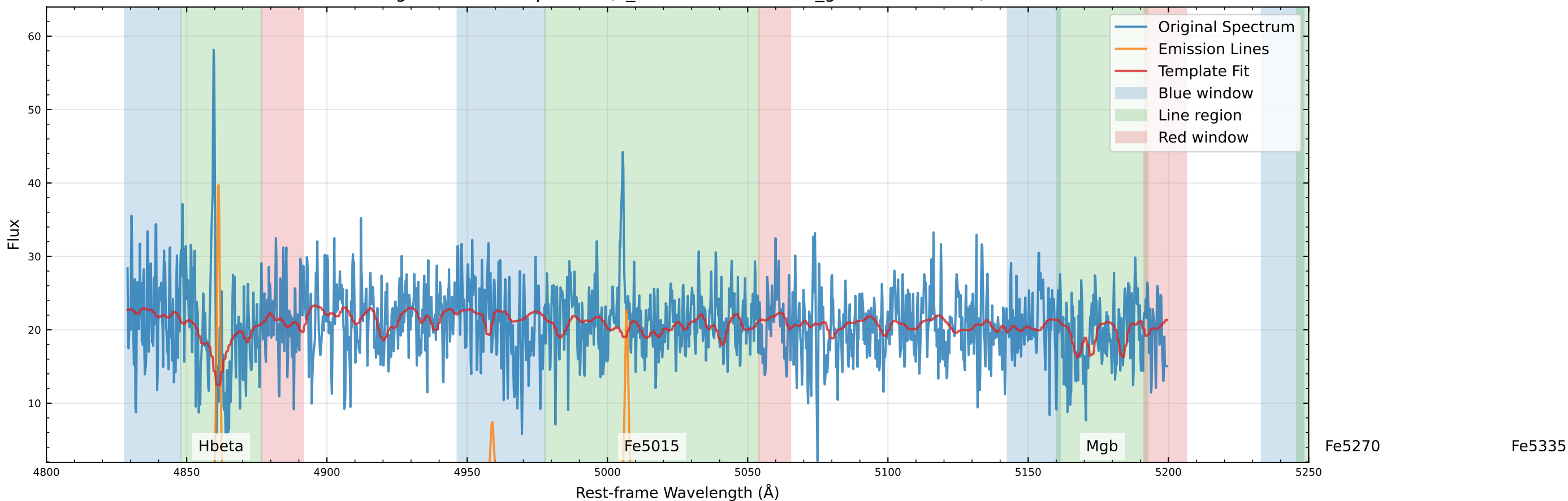
Original Data Comparison (v_star=-116.5 km/s, v_gas=-107.3 km/s)
